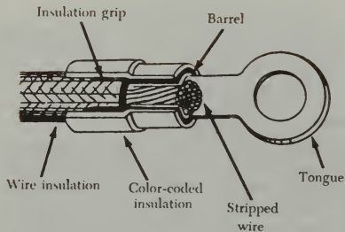
FIGURE 4-106. Preinsulated terminal lug.
